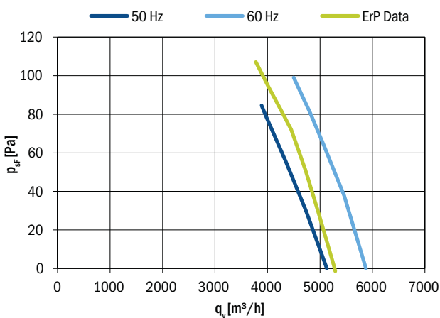
Fan characteristic measured in short bell mouth with guard grill characteristic measured in full bell mouth without guard grill
